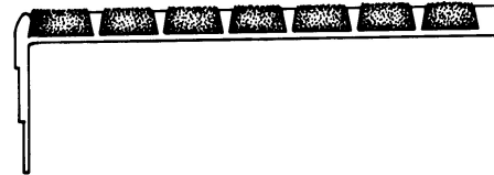
Type 142 4" wide, 1/4" thick, nose 1 1/8" underside DRAWING NOT TO SCALE
