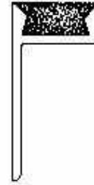
Type WP1SP 3/4" wide, 3/8" thick, 1 1/2" overall DRAWING NOT TO SCALE
