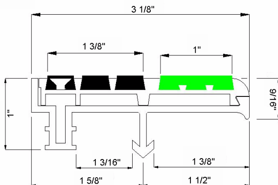
Detail - sure hold anchor in concrete step
